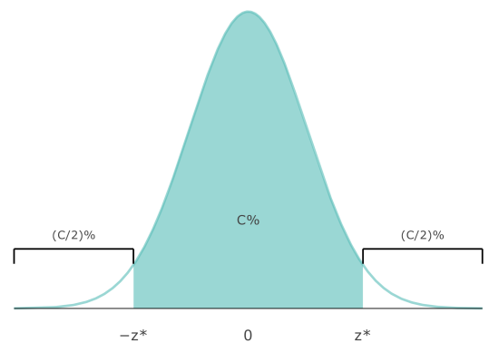
Figure 5.2: The central area under the standard normal curve with confidence level C .
